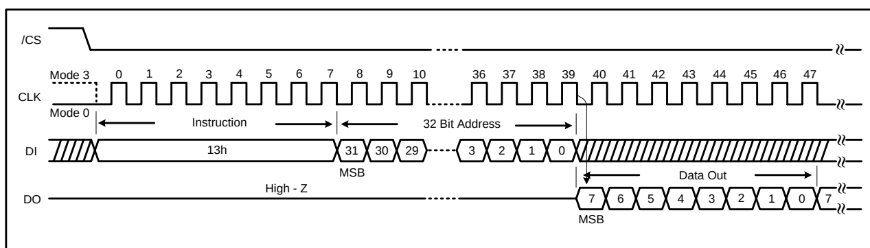
Figure 15. Read Data with 4-Byte Address Instruction
