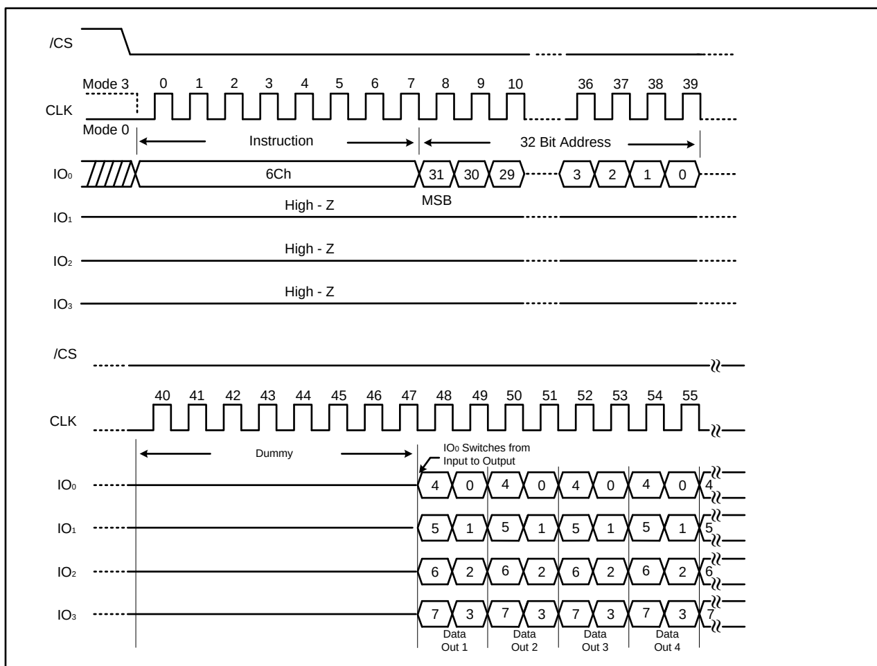
Figure 21. Fast Read Quad Output with 4-Byte Address Instruction
