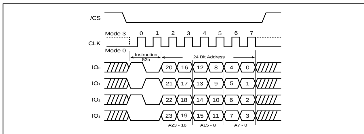
Figure 36b. 32KB Block Erase Instruction (QPI Mode)
