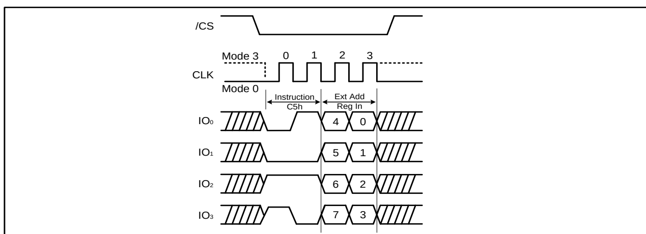
Figure 11b. Write Extended Address Register Instruction (QPI Mode)
