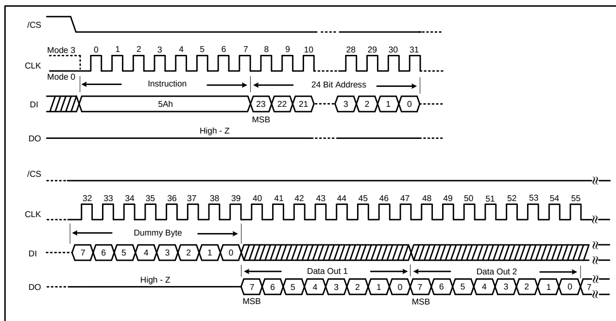
Figure 49. Read SFDP Register Instruction Sequence Diagram
