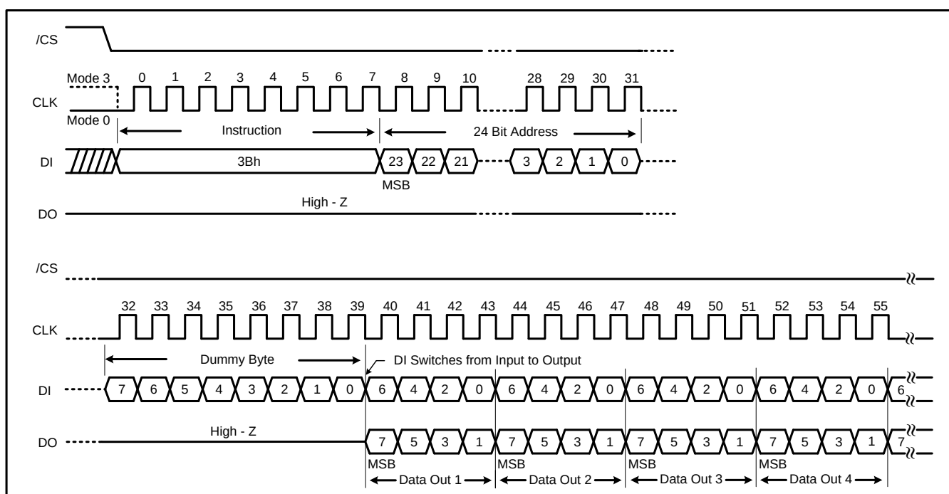
Figure 18. Fast Read Dual Output Instruction
