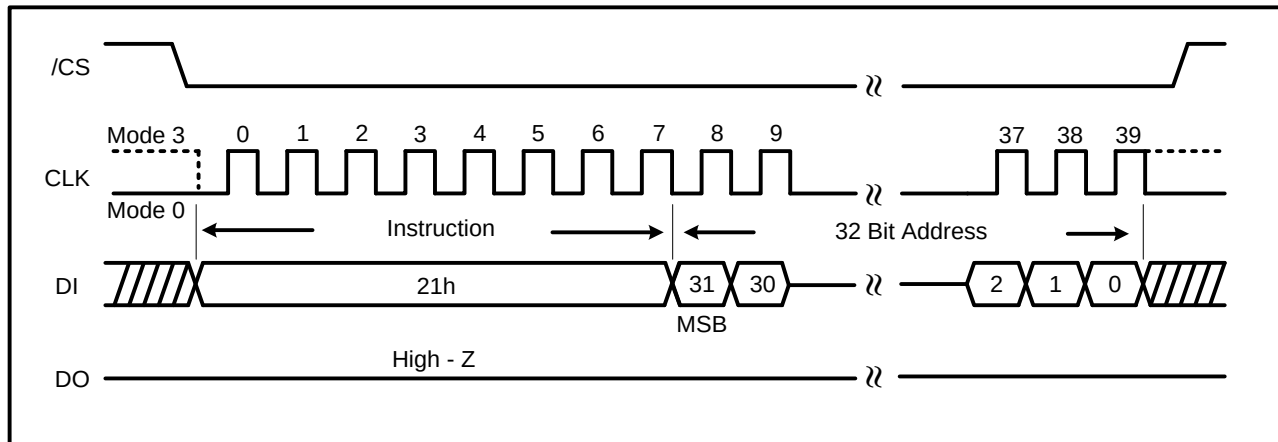
Figure 35. Sector Erase with 4-Byte Address Instruction
