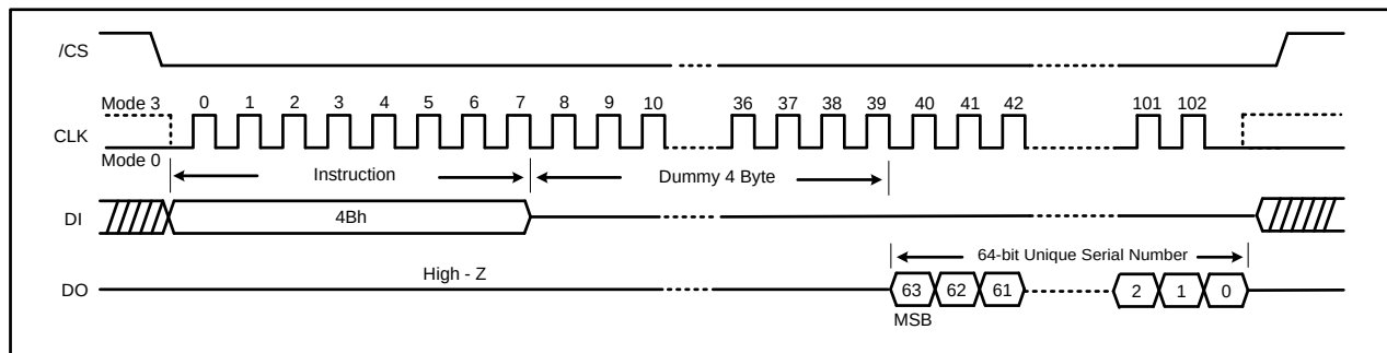
Figure 47. Read Unique ID Number Instruction (SPI Mode only)
