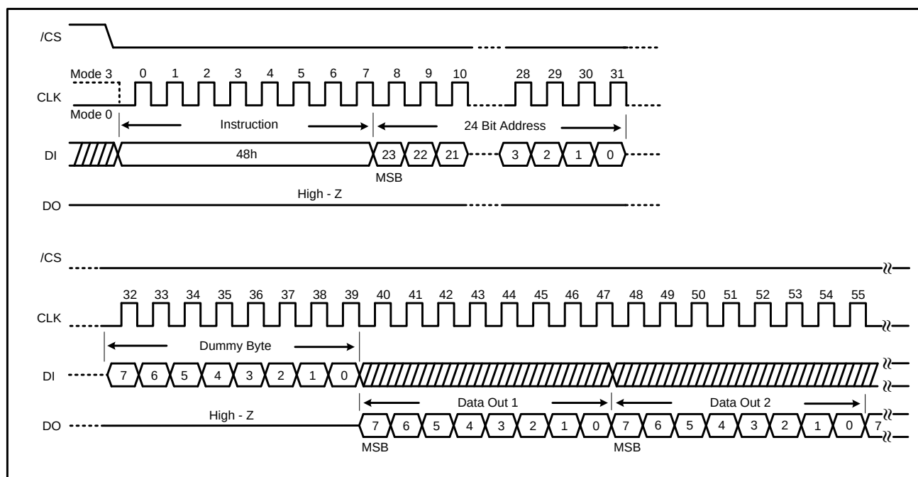
Figure 52. Read Security Registers Instruction (SPI Mode only)
