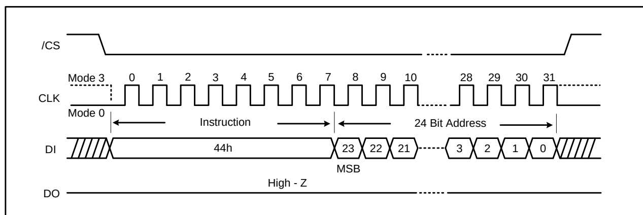
Figure 50. Erase Security Registers Instruction (SPI Mode only)
