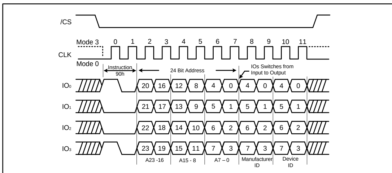
Figure 44b. Read Manufacturer / Device ID Instruction (QPI Mode)
