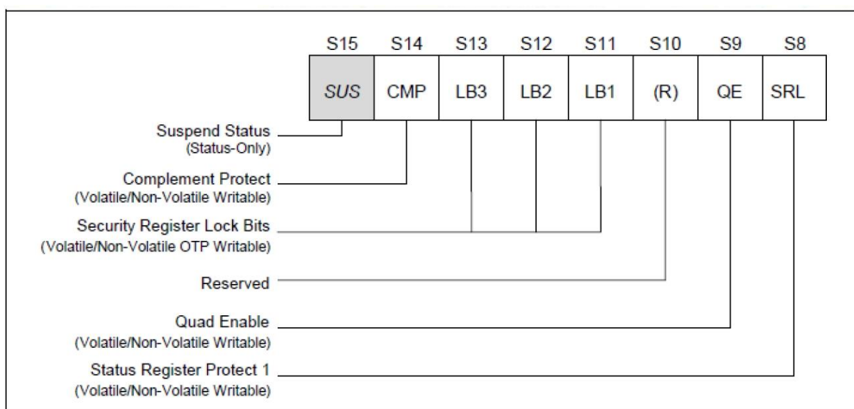
Figure 4c. Status Register-2
