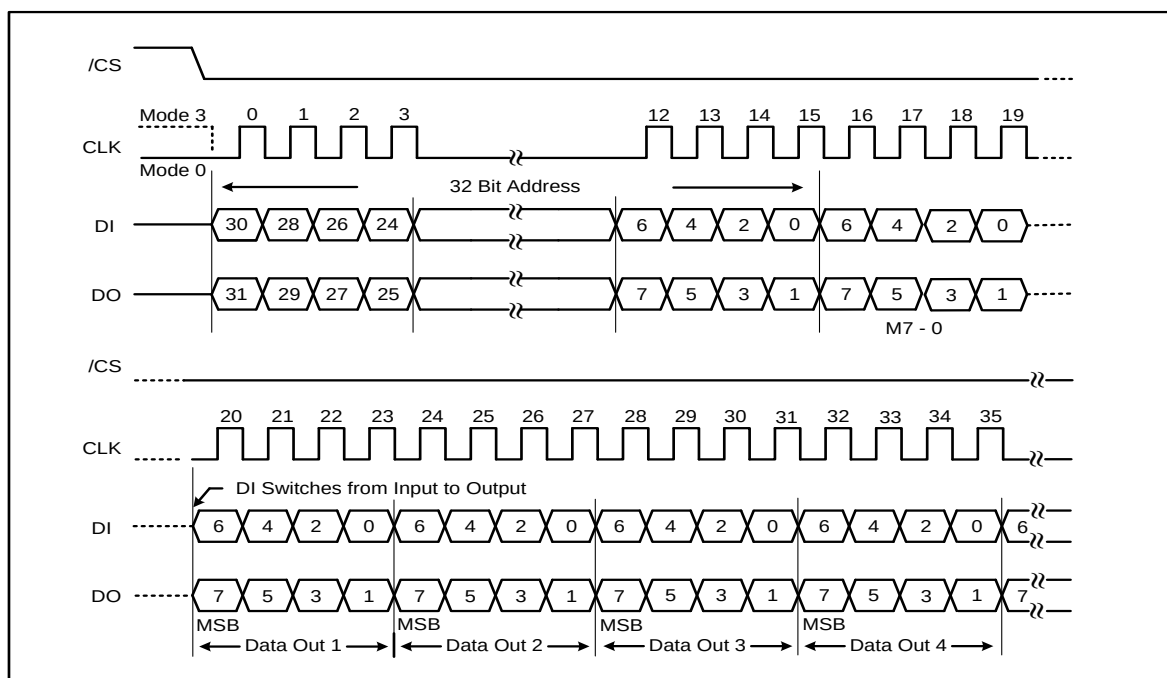
Figure 23b. Fast Read Dual I/O with 4-Byte Address Instruction. (Previous instruction set M5-4 0, SPI Mode only)
