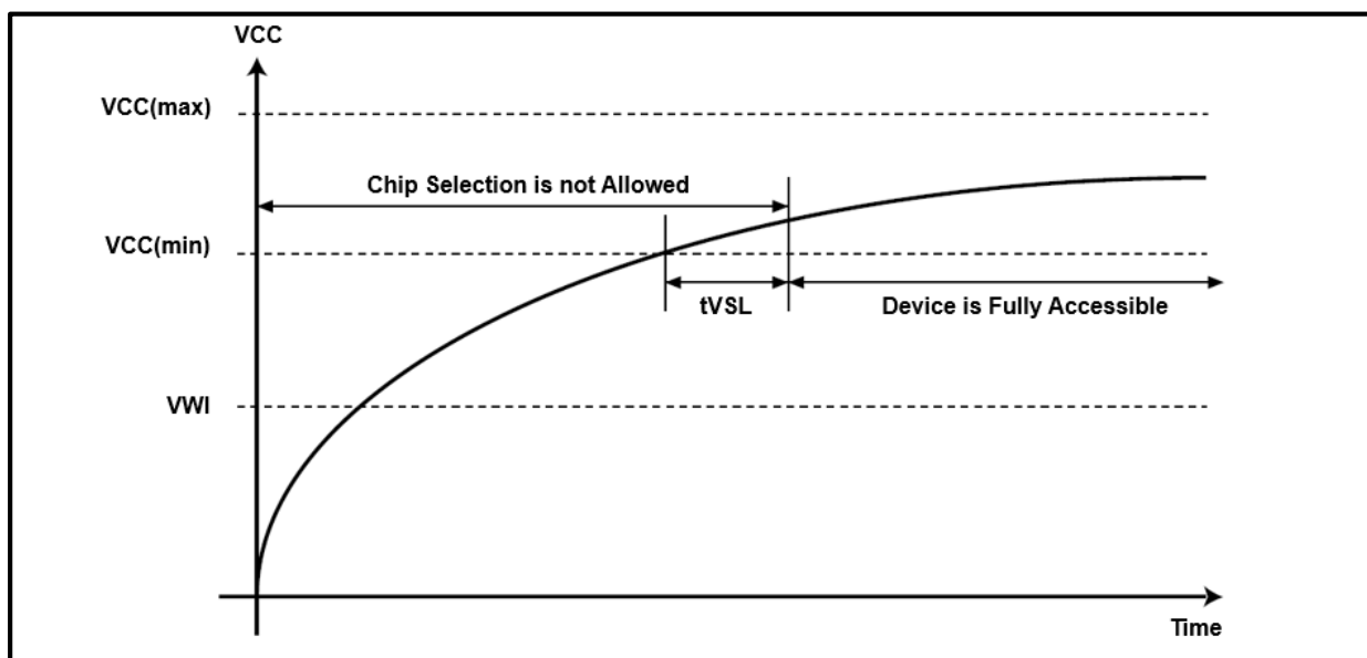
Figure 58a. Power-up Timing and Voltage Levels
