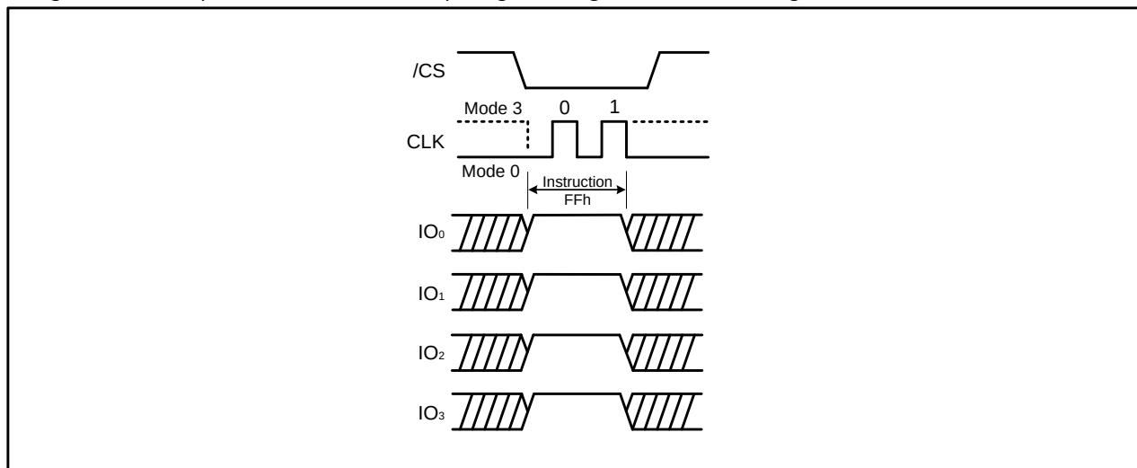
Figure 56. Exit QPI Instruction (QPI Mode only)
