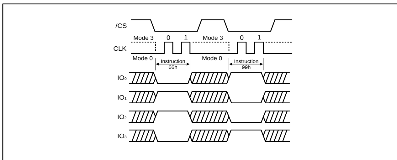
Figure 57b. Enable Reset and Reset Instruction Sequence (QPI Mode)
