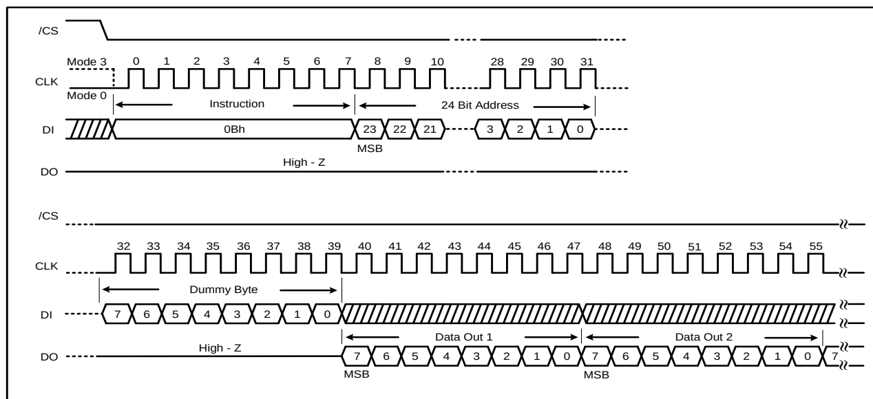
Figure 16a. Fast Read Instruction (SPI Mode)
