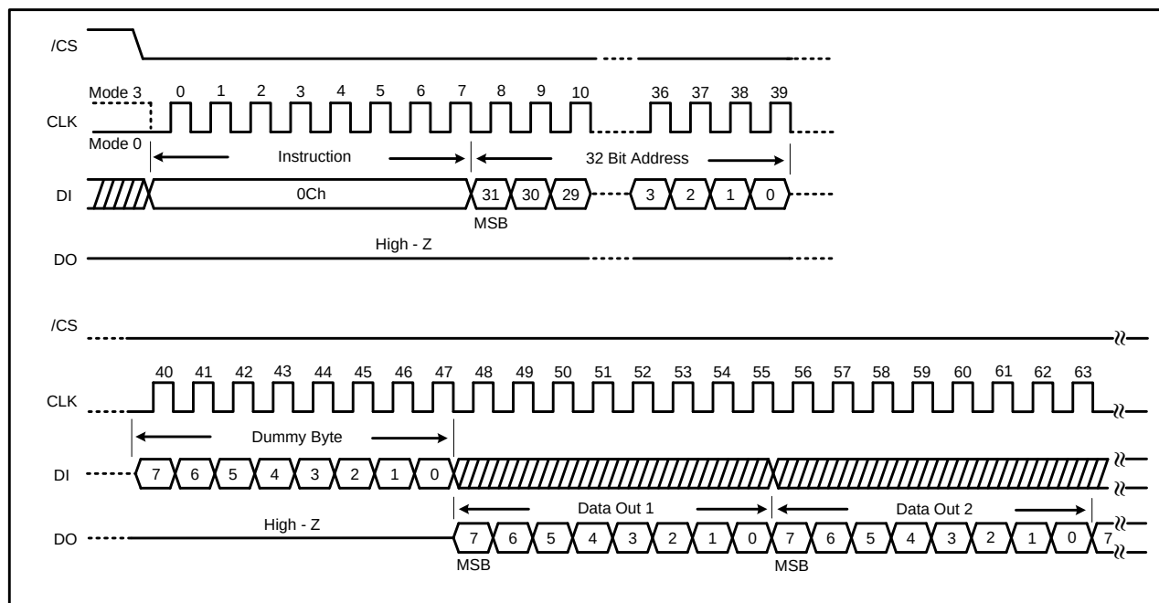
Figure 17. Fast Read with 4-Byte Address Instruction
