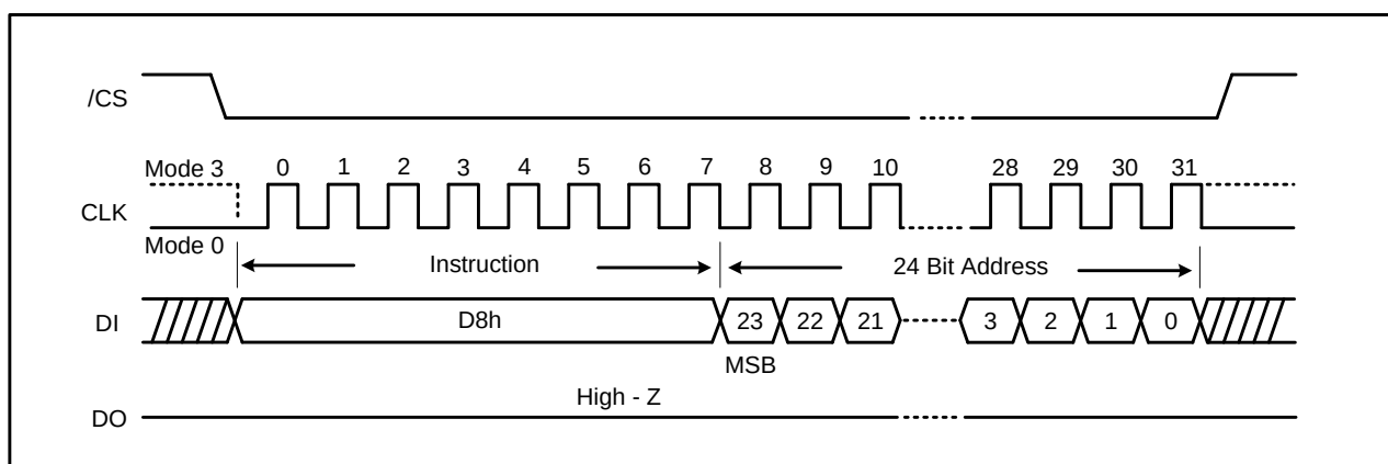
Figure 37a. 64KB Block Erase Instruction (SPI Mode)
