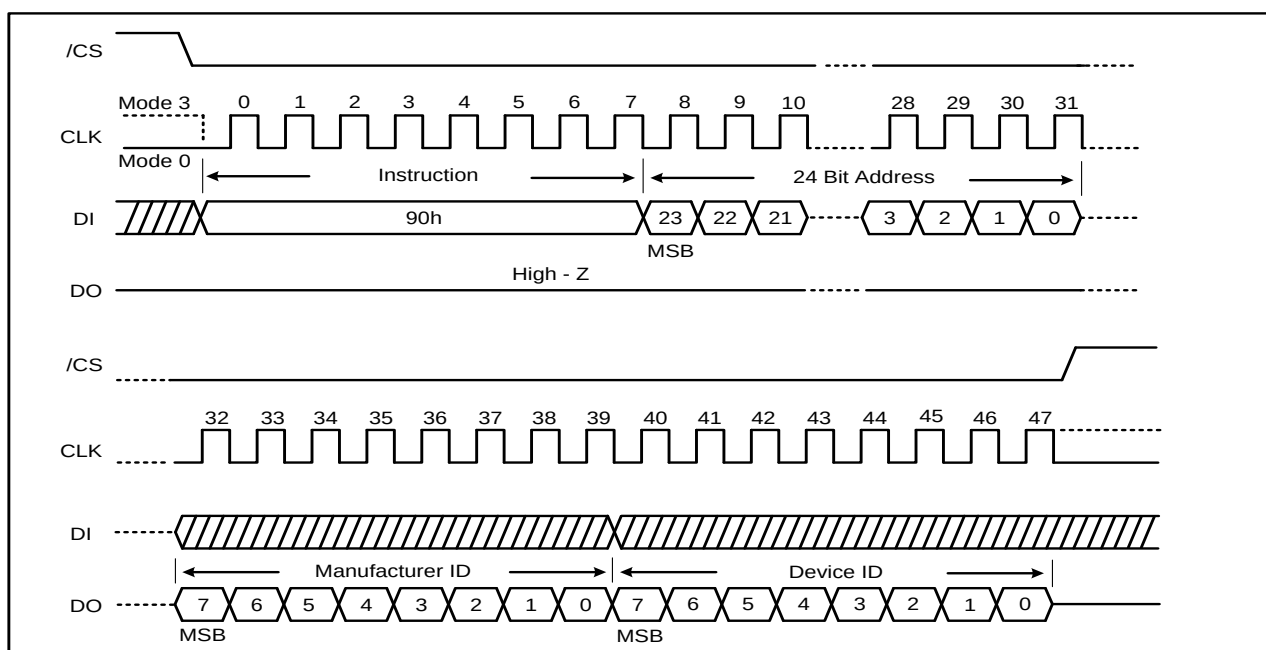
Figure 44a. Read Manufacturer / Device ID Instruction (SPI Mode)
